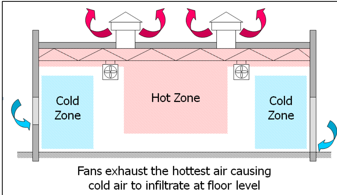
Figure 13: Air Temperature Stratification in Large Industrial Buildings
